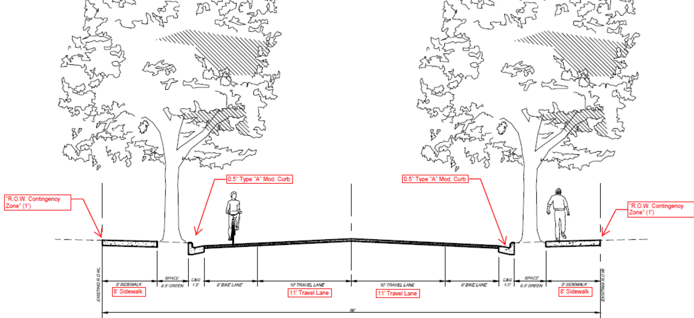
TYPICAL SECTION - UNIVERSITY BLVD. QUEEN CITY AVE. EAST TO GENE STALLINGS AVE.
