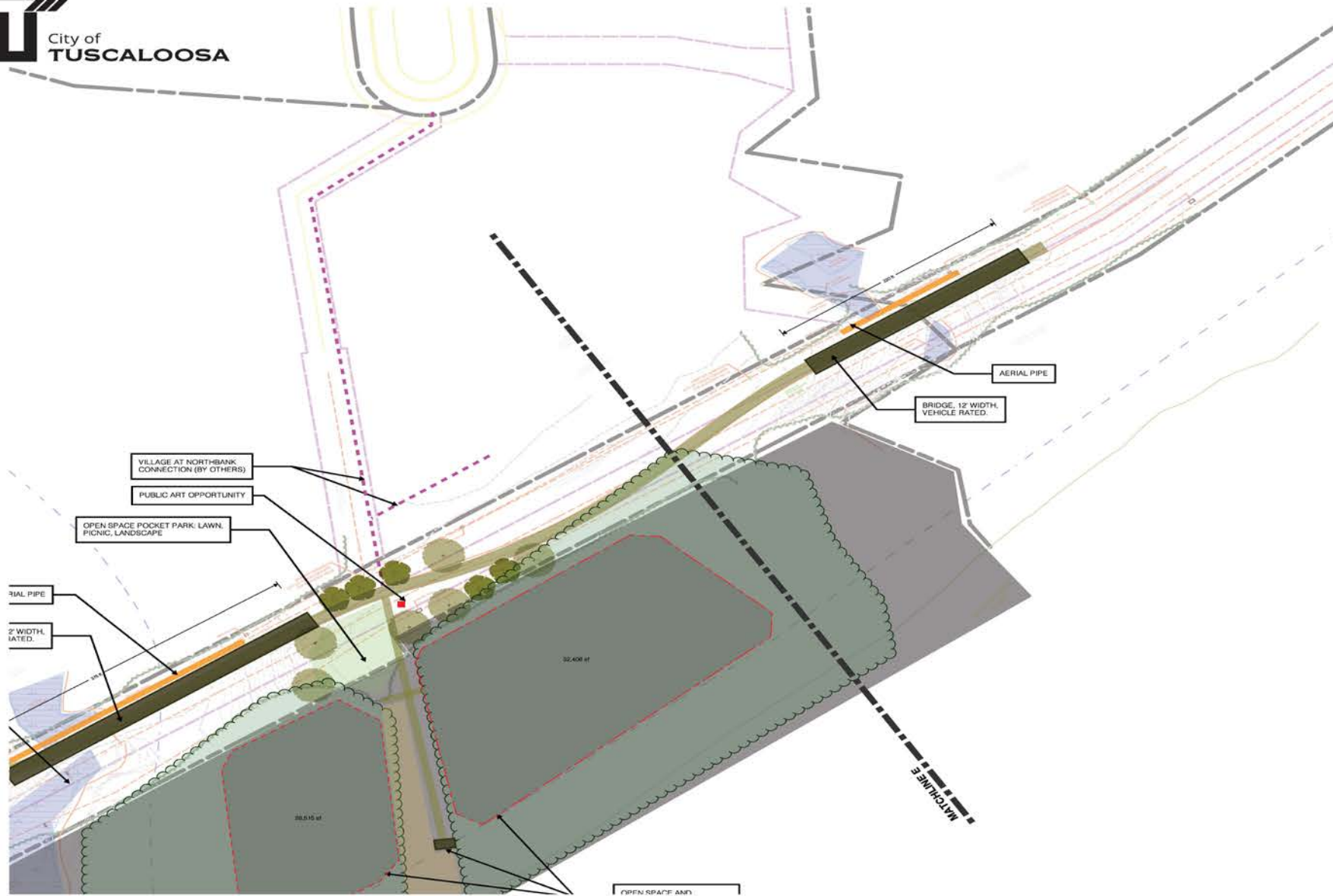
CITY OF TUSCALOOSA NORTHERN RIVERWALK - RANDALL PARK + TRAILHEAD - SCHEMATIC DESIGN JANUARY 29, 2020
